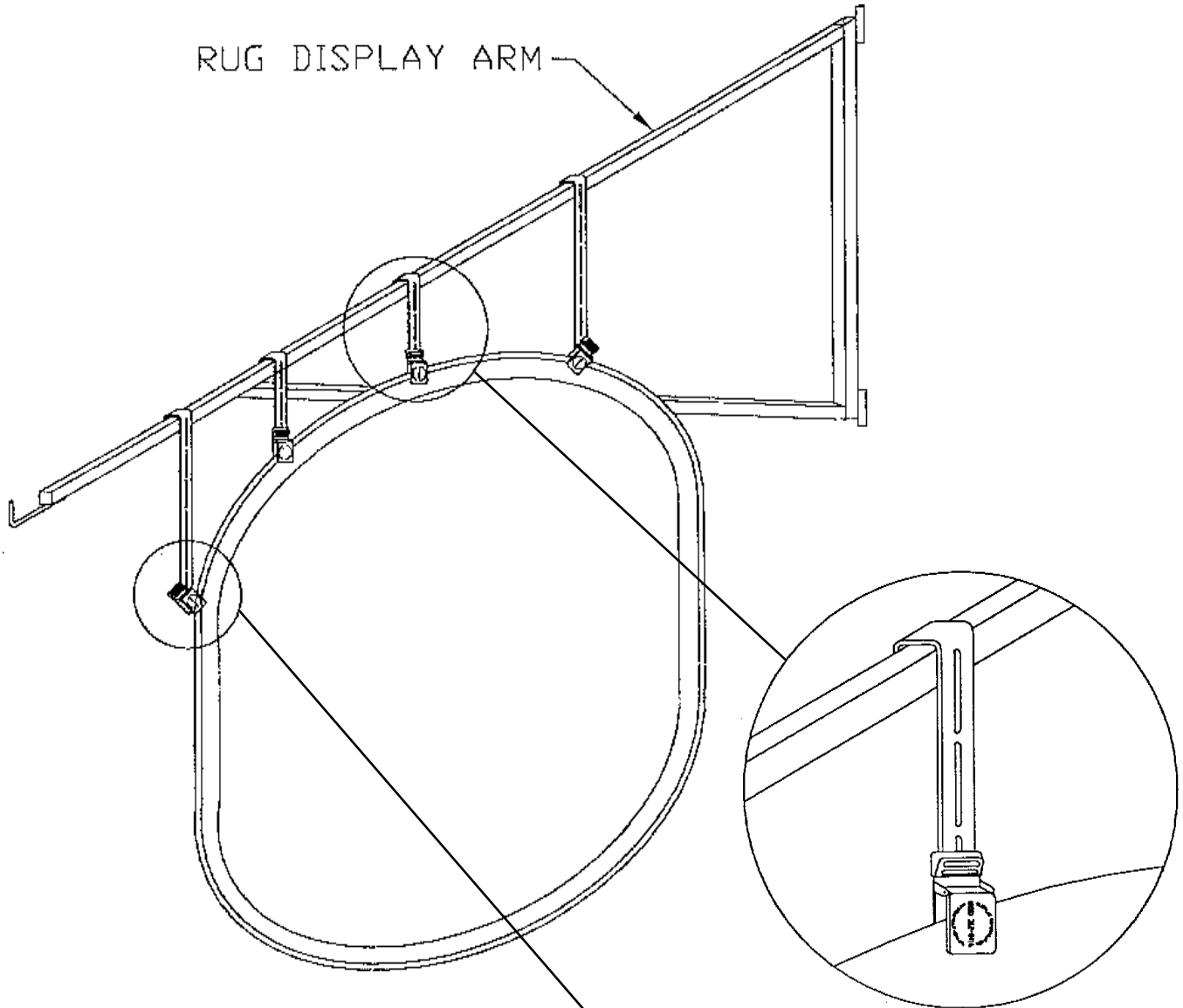
Oval Rug Hanger
